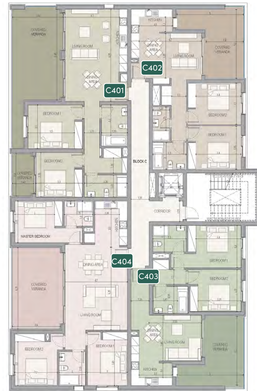
BLOCK C 4th FLOOR PLAN 1:100
